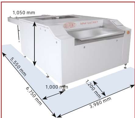
Technical Drawing
